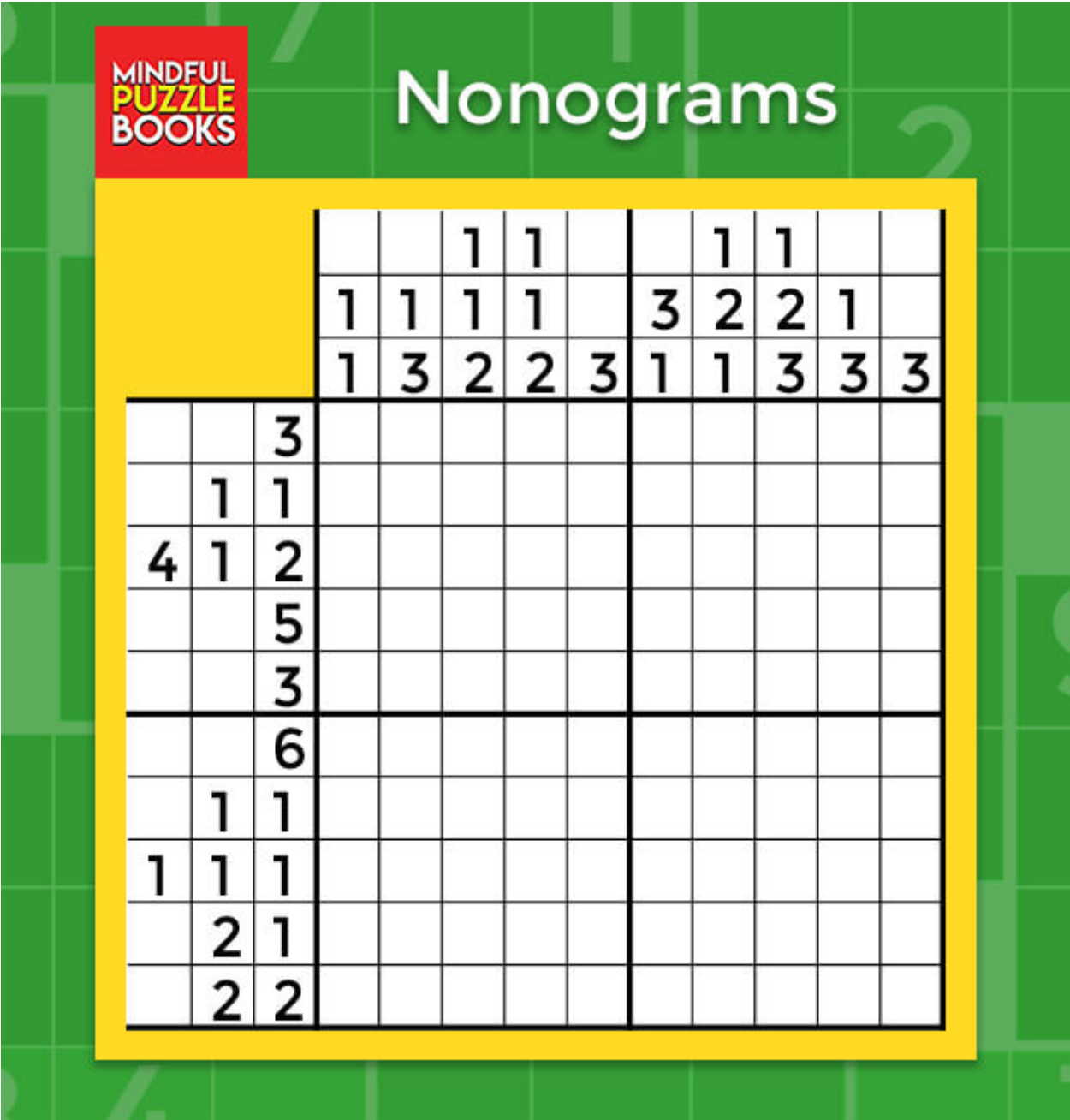
Nonograms
